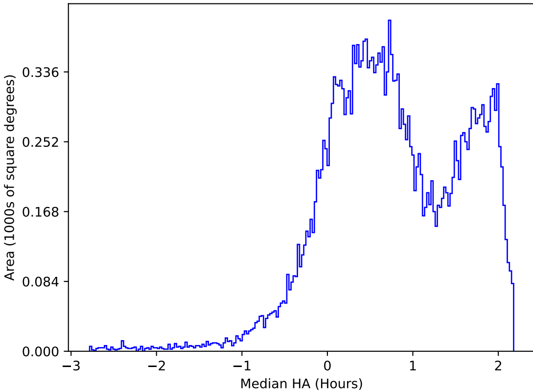
too_elab_r8_d2_gz_v3.4_10yrs All sky r band: Median HA
