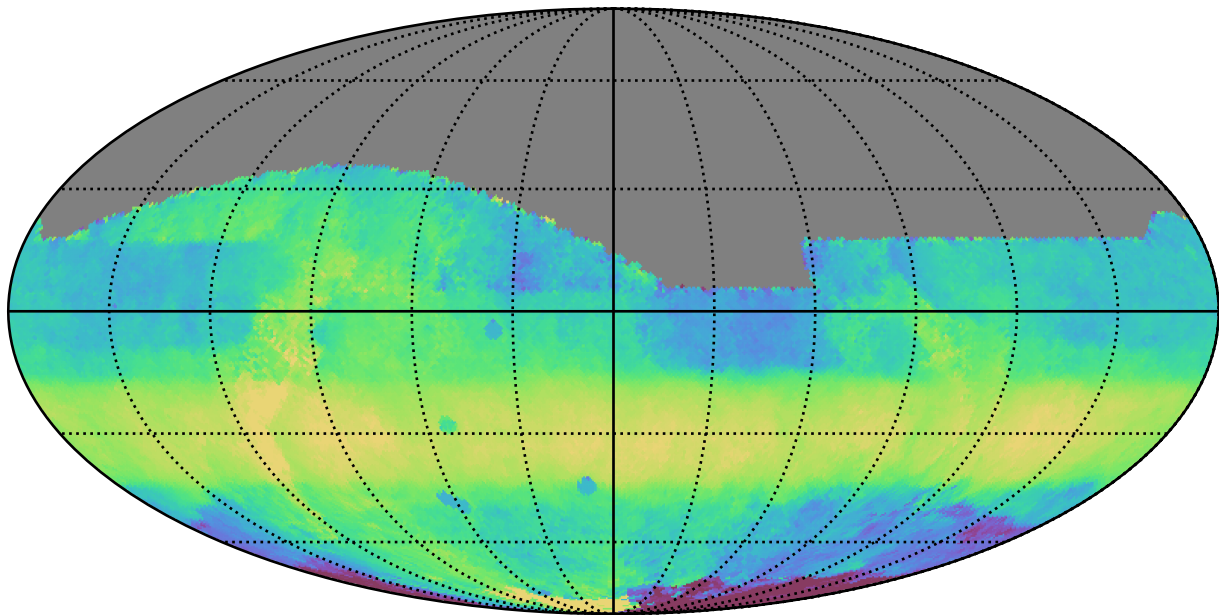
too_elab_r8_d2_gz_v3.4_10yrs All sky i band: Median HA
