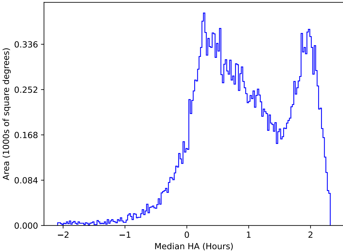
too_elab_r8_d2_gz_v3.4_10yrs All sky i band: Median HA
