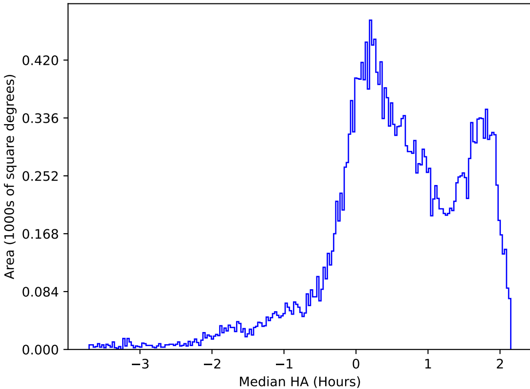
too_elab_r8_d2_gz_v3.4_10yrs All sky g band: Median HA
