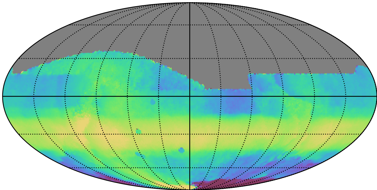
too_elab_r8_d2_gz_v3.4_10yrs All sky all bands: Median HA
