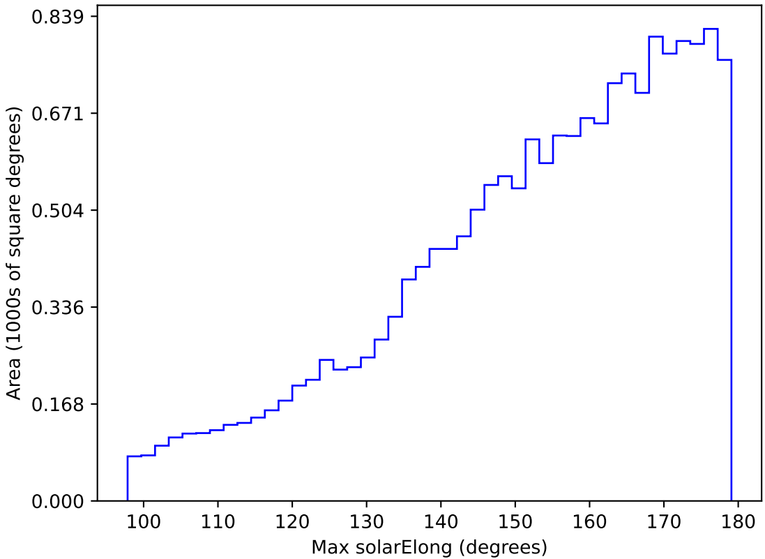
too_elab_r8_d2_gz_v3.4_10yrs WFD u band: Max solarElong
