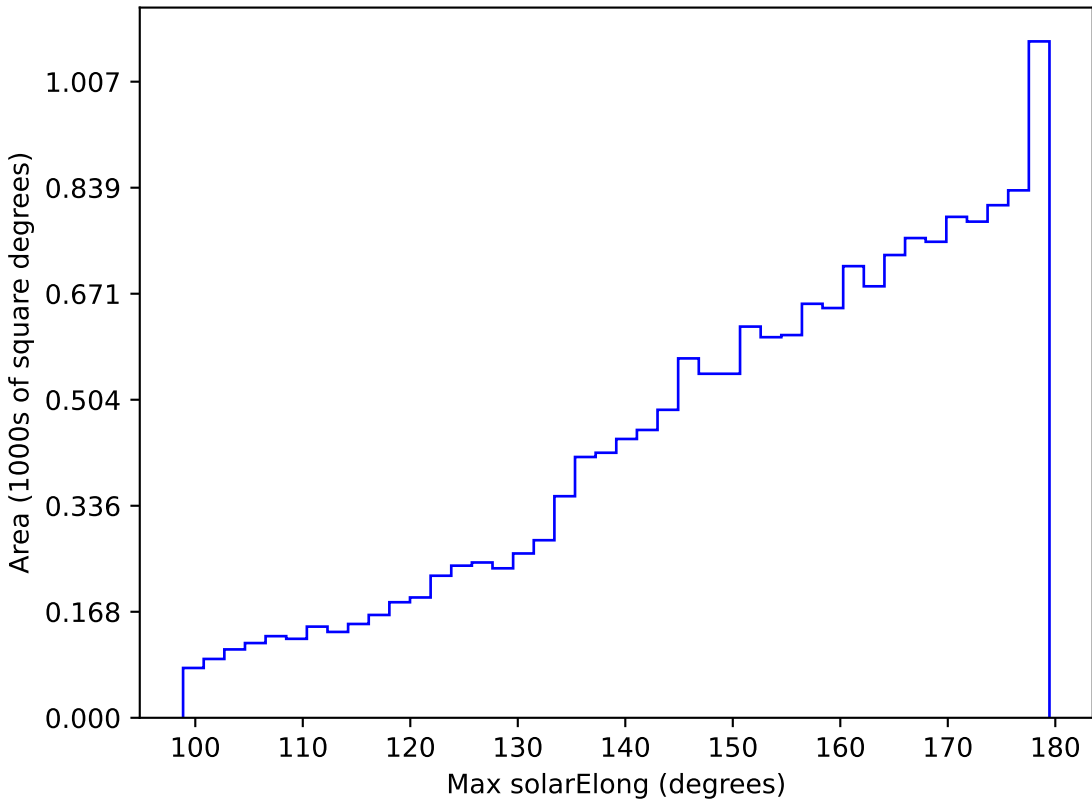
too_elab_r8_d2_gz_v3.4_10yrs WFD r band: Max solarElong
