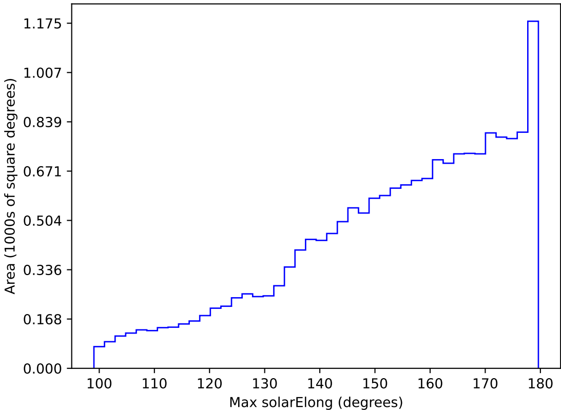
too_elab_r8_d2_gz_v3.4_10yrs WFD all bands: Max solarElong
