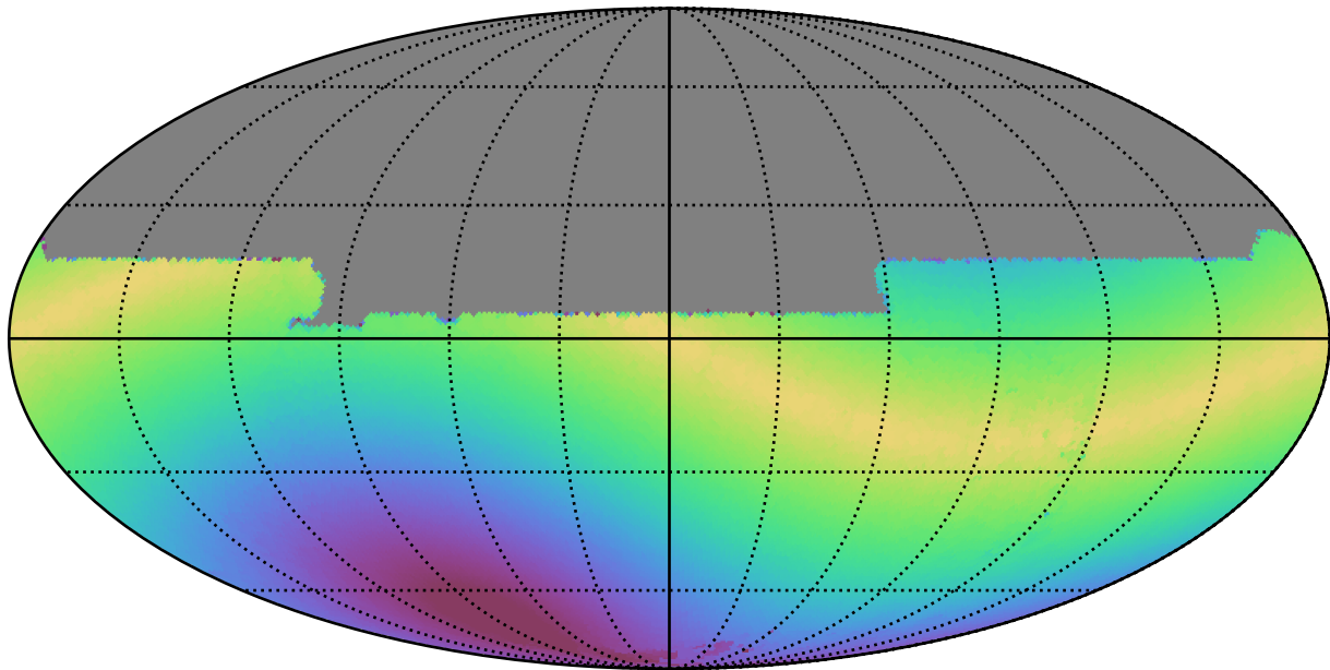
too_elab_r8_d2_gz_v3.4_10yrs All sky y band: Max solarElong
