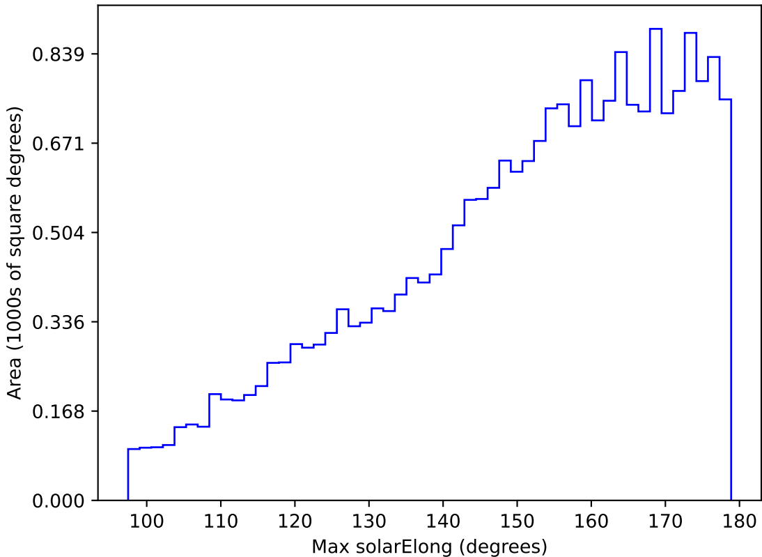
too_elab_r8_d2_gz_v3.4_10yrs All sky u band: Max solarElong
