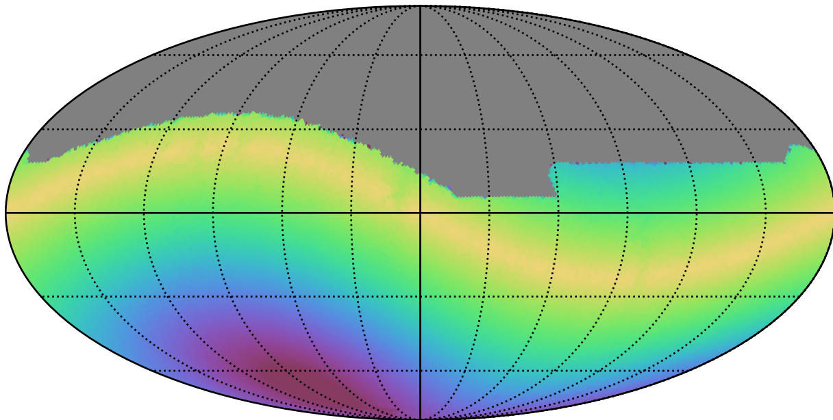
too_elab_r8_d2_gz_v3.4_10yrs All sky r band: Max solarElong
