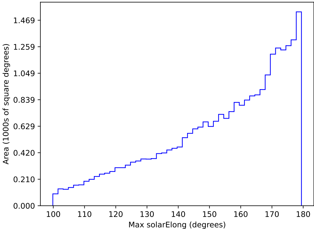
too_elab_r8_d2_gz_v3.4_10yrs All sky r band: Max solarElong
