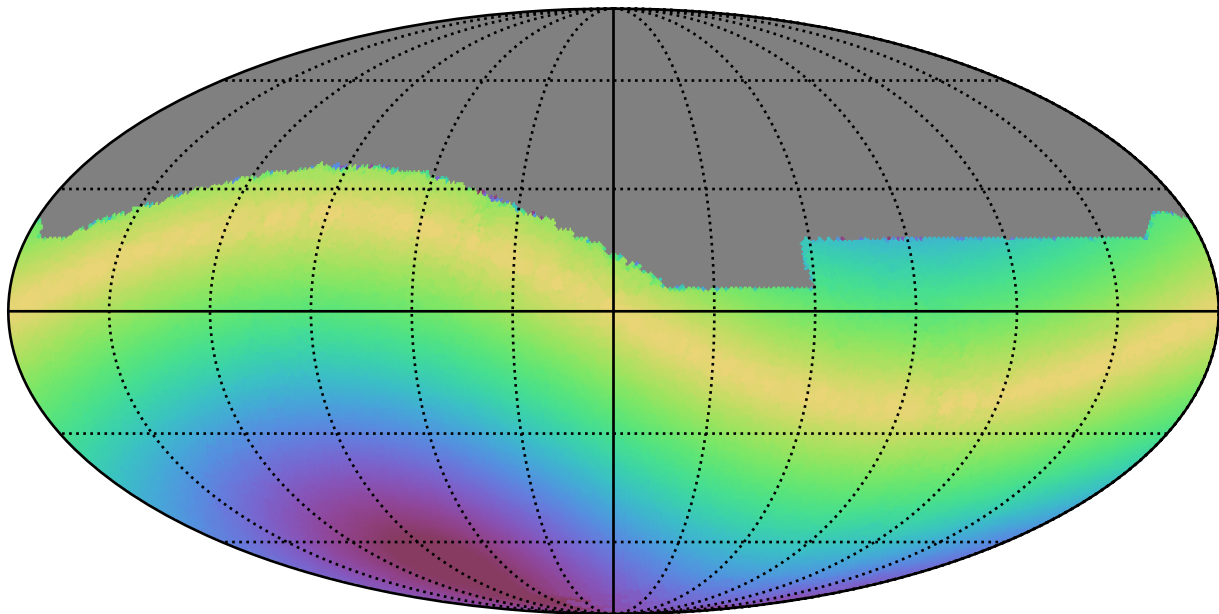
too_elab_r8_d2_gz_v3.4_10yrs All sky i band: Max solarElong
