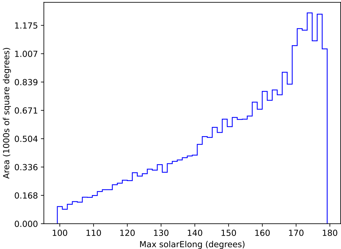
too_elab_r8_d2_gz_v3.4_10yrs All sky g band: Max solarElong
