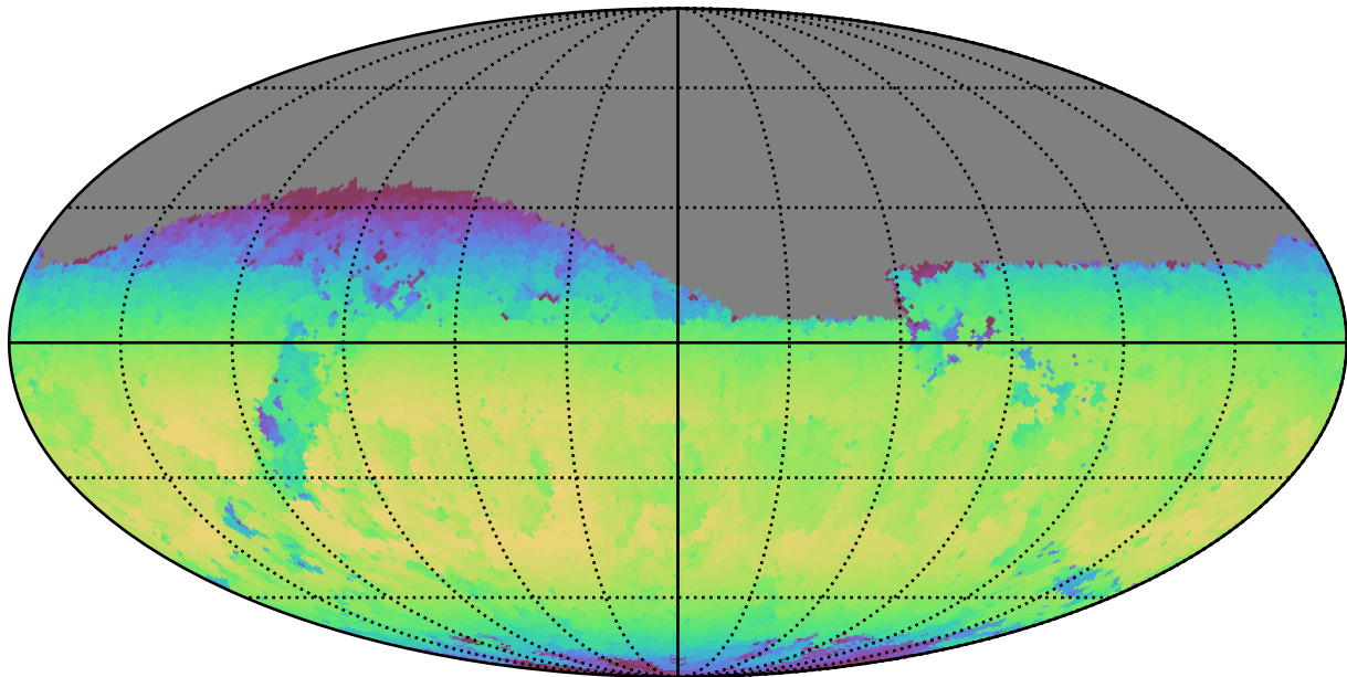
too_elab_r8_d2_gz_v3.4_10yrs Yr 1 z band: Max skyBrightness
