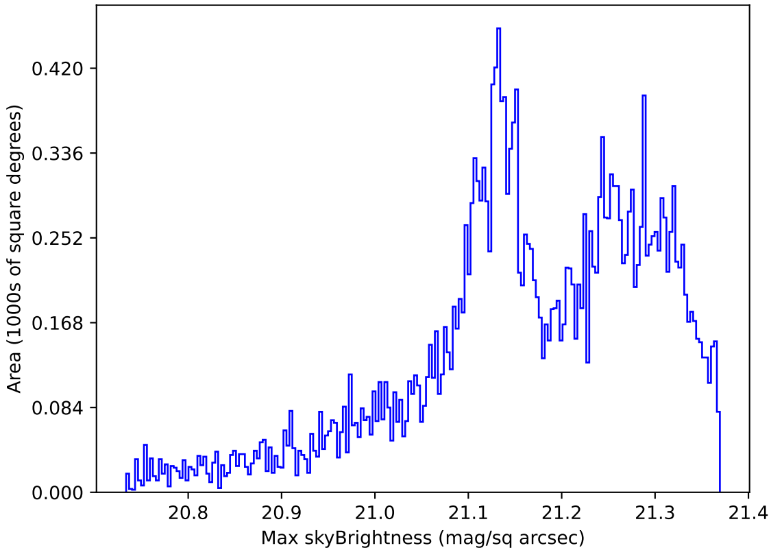
too_elab_r8_d2_gz_v3.4_10yrs Yr 1 r band: Max skyBrightness
