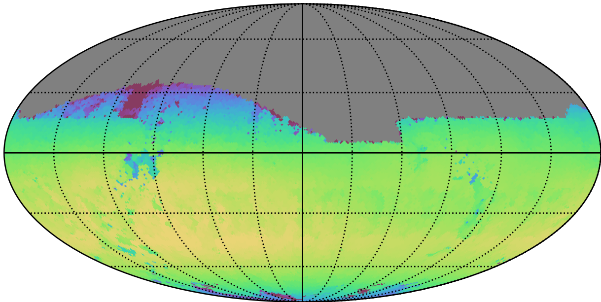
too_elab_r8_d2_gz_v3.4_10yrs Yr 1 i band: Max skyBrightness
