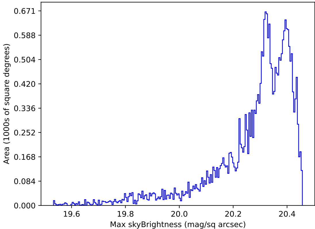
too_elab_r8_d2_gz_v3.4_10yrs Yr 1 i band: Max skyBrightness
