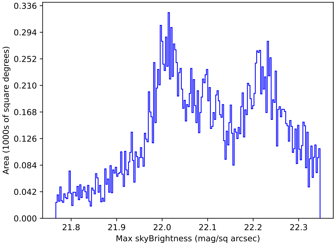
too_elab_r8_d2_gz_v3.4_10yrs Yr 1 g band: Max skyBrightness
