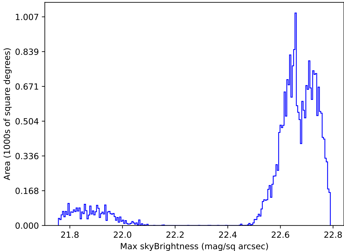
too_elab_r8_d2_gz_v3.4_10yrs Yr 1 all bands: Max skyBrightness
