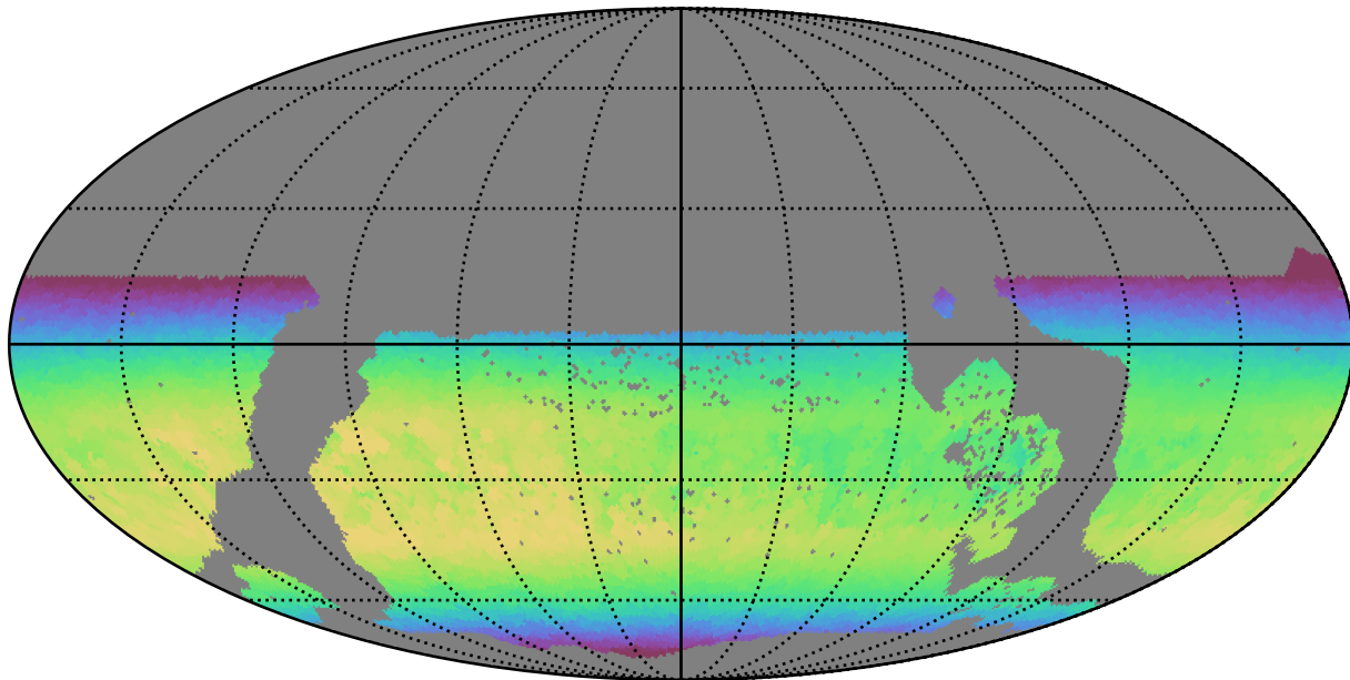
too_elab_r8_d2_gz_v3.4_10yrs WFD z band: Max skyBrightness
