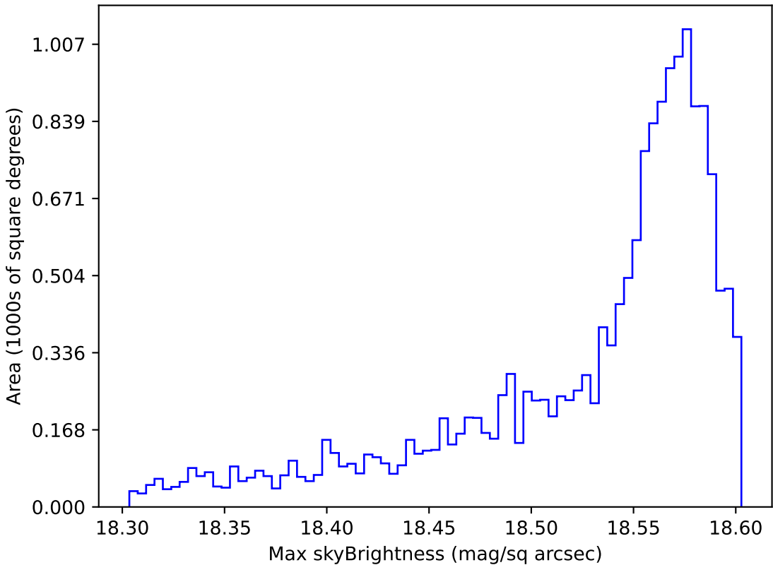
too_elab_r8_d2_gz_v3.4_10yrs WFD y band: Max skyBrightness
