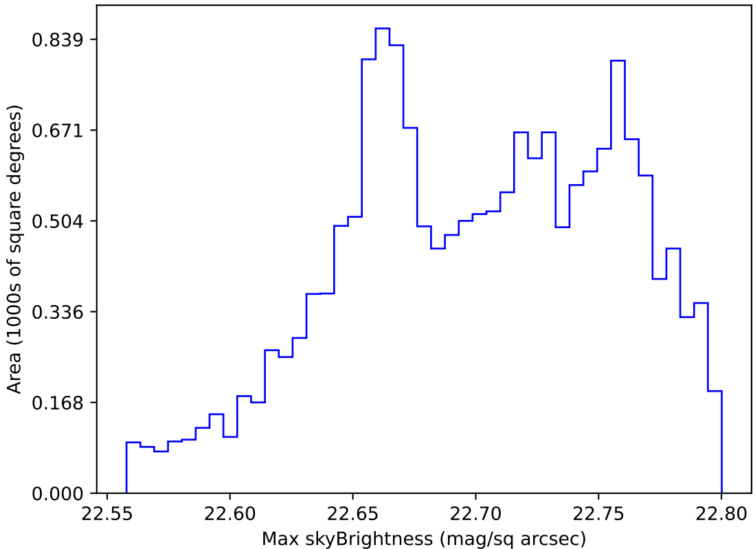
too_elab_r8_d2_gz_v3.4_10yrs WFD u band: Max skyBrightness
