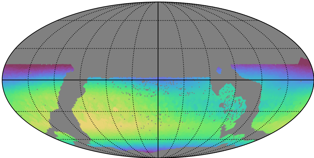
too_elab_r8_d2_gz_v3.4_10yrs WFD i band: Max skyBrightness
