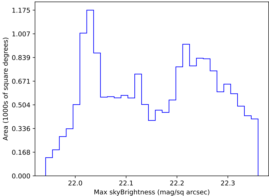
too_elab_r8_d2_gz_v3.4_10yrs WFD g band: Max skyBrightness
