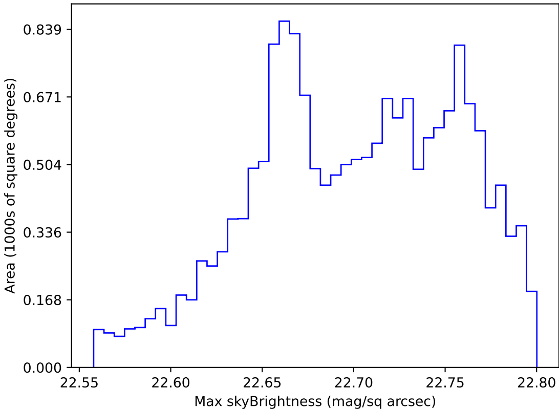
too_elab_r8_d2_gz_v3.4_10yrs WFD all bands: Max skyBrightness
