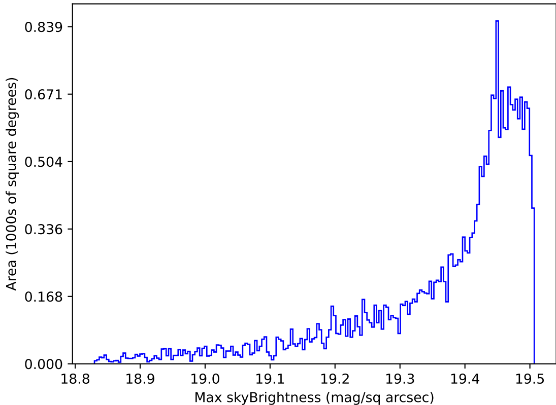
too_elab_r8_d2_gz_v3.4_10yrs All sky z band: Max skyBrightness
