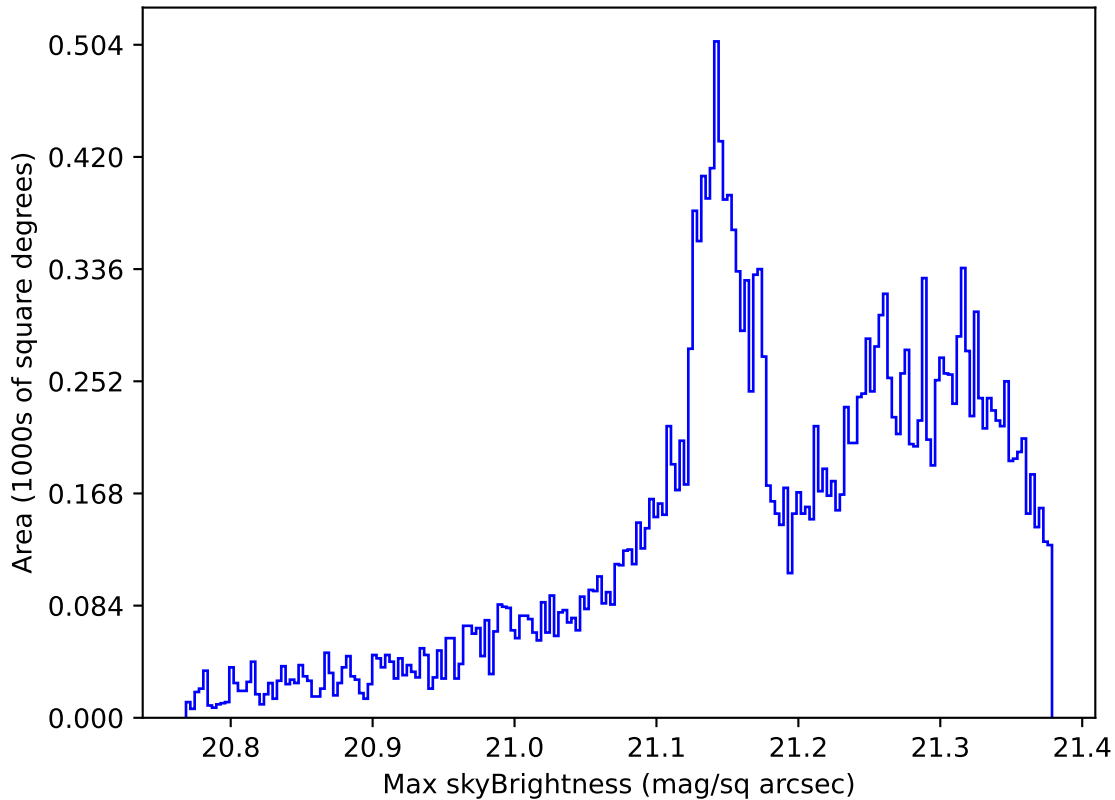
too_elab_r8_d2_gz_v3.4_10yrs All sky r band: Max skyBrightness
