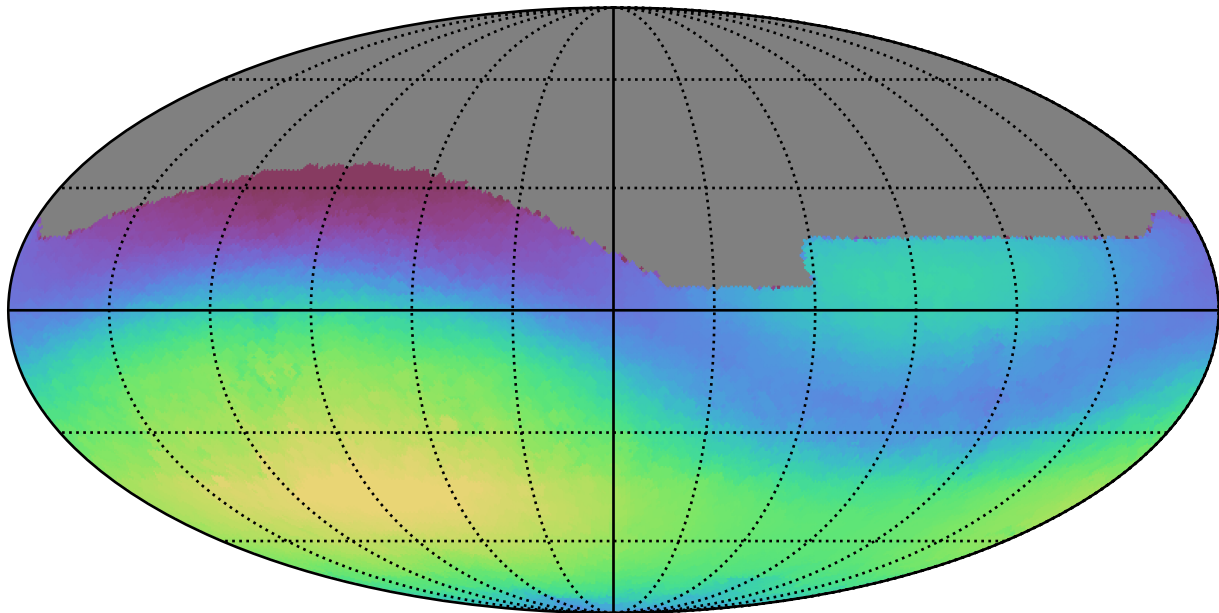
too_elab_r8_d2_gz_v3.4_10yrs All sky g band: Max skyBrightness
