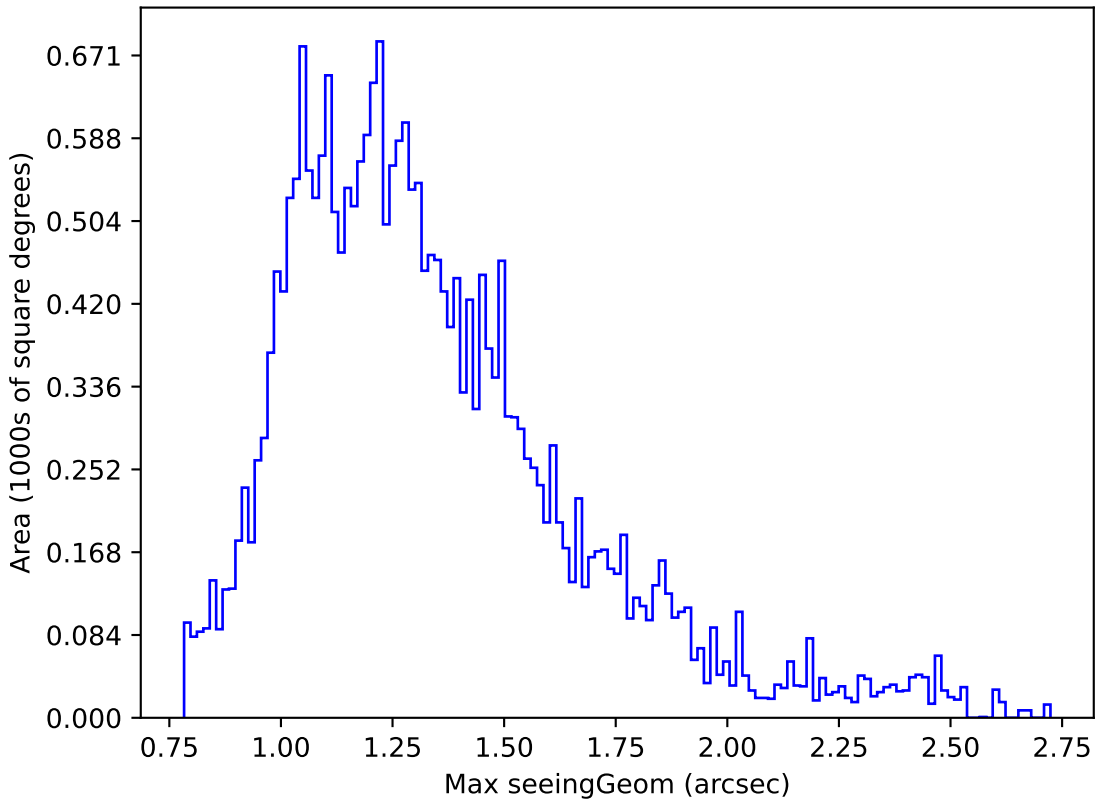
too_elab_r8_d2_gz_v3.4_10yrs Yr 1 z band: Max seeingGeom
