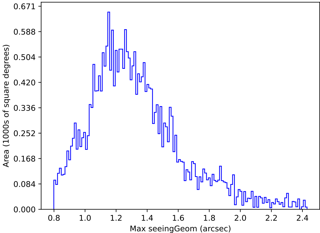
too_elab_r8_d2_gz_v3.4_10yrs Yr 1 g band: Max seeingGeom
