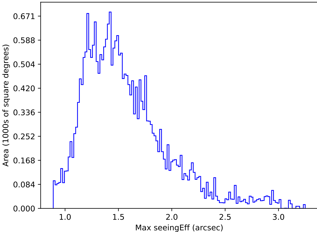
too_elab_r8_d2_gz_v3.4_10yrs Yr 1 z band: Max seeingEff
