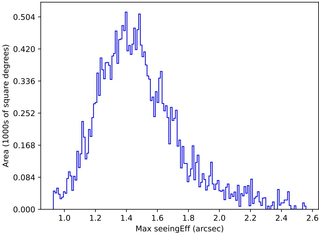
too_elab_r8_d2_gz_v3.4_10yrs Yr 1 y band: Max seeingEff
