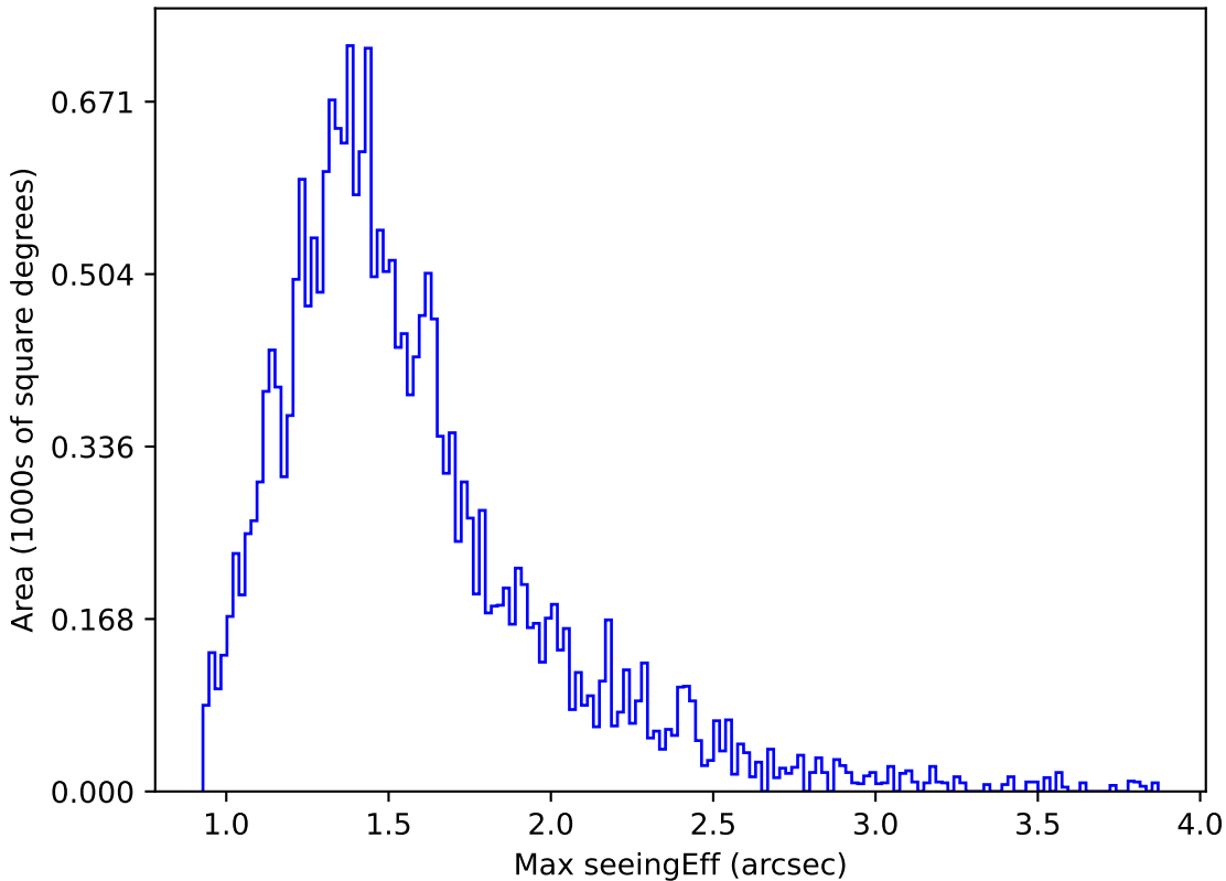
too_elab_r8_d2_gz_v3.4_10yrs Yr 1 u band: Max seeingEff
