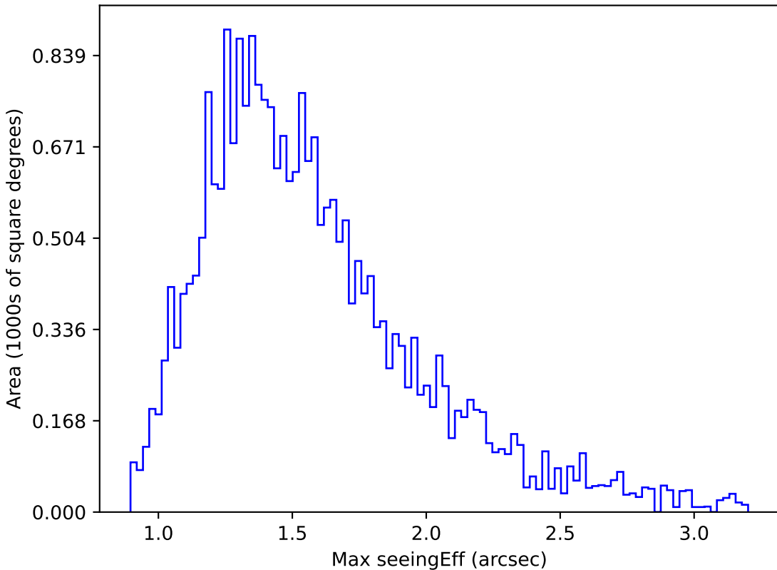
too_elab_r8_d2_gz_v3.4_10yrs Yr 1 i band: Max seeingEff
