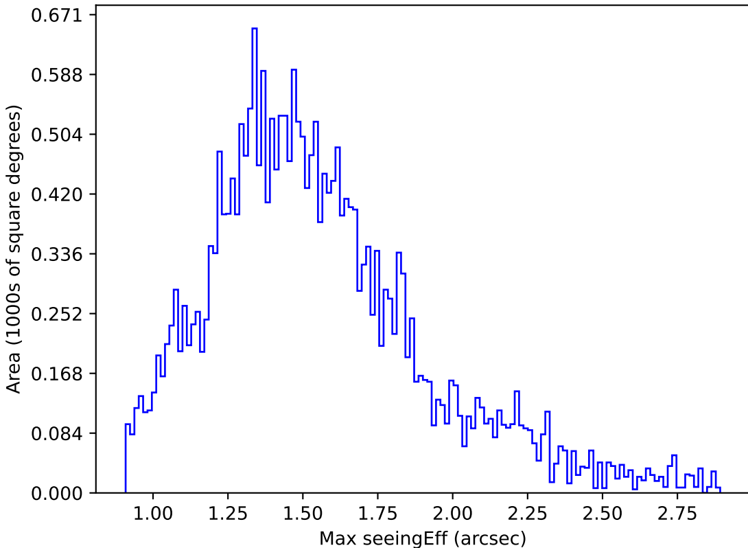
too_elab_r8_d2_gz_v3.4_10yrs Yr 1 g band: Max seeingEff
