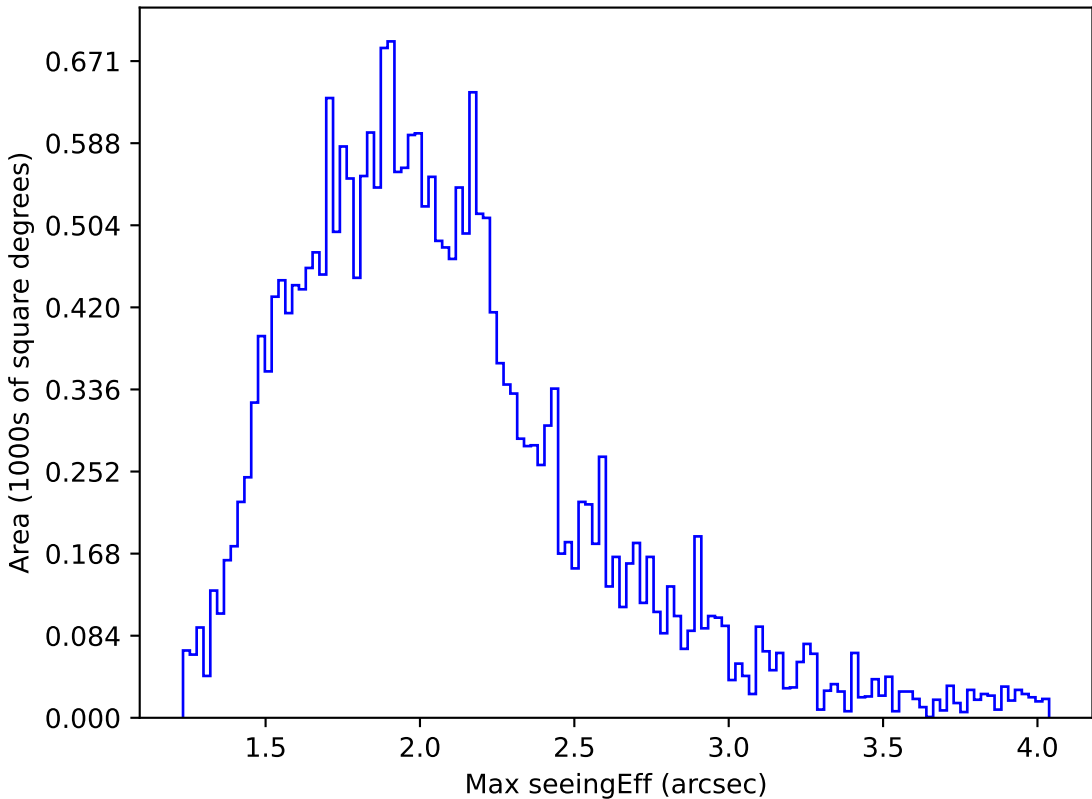
too_elab_r8_d2_gz_v3.4_10yrs Yr 1 all bands: Max seeingEff
