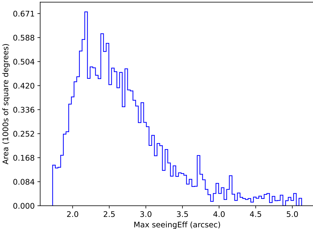
too_elab_r8_d2_gz_v3.4_10yrs WFD z band: Max seeingEff
