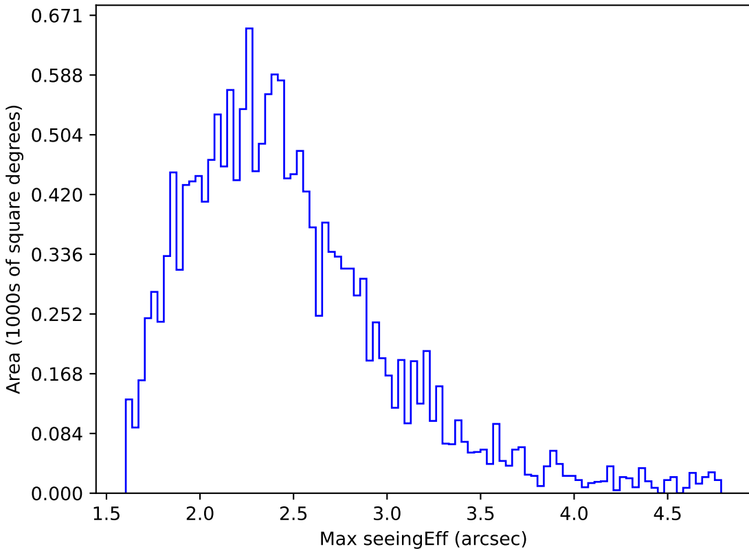
too_elab_r8_d2_gz_v3.4_10yrs WFD y band: Max seeingEff
