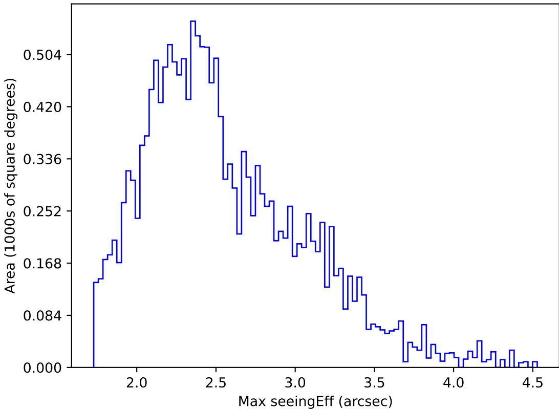
too_elab_r8_d2_gz_v3.4_10yrs WFD u band: Max seeingEff
