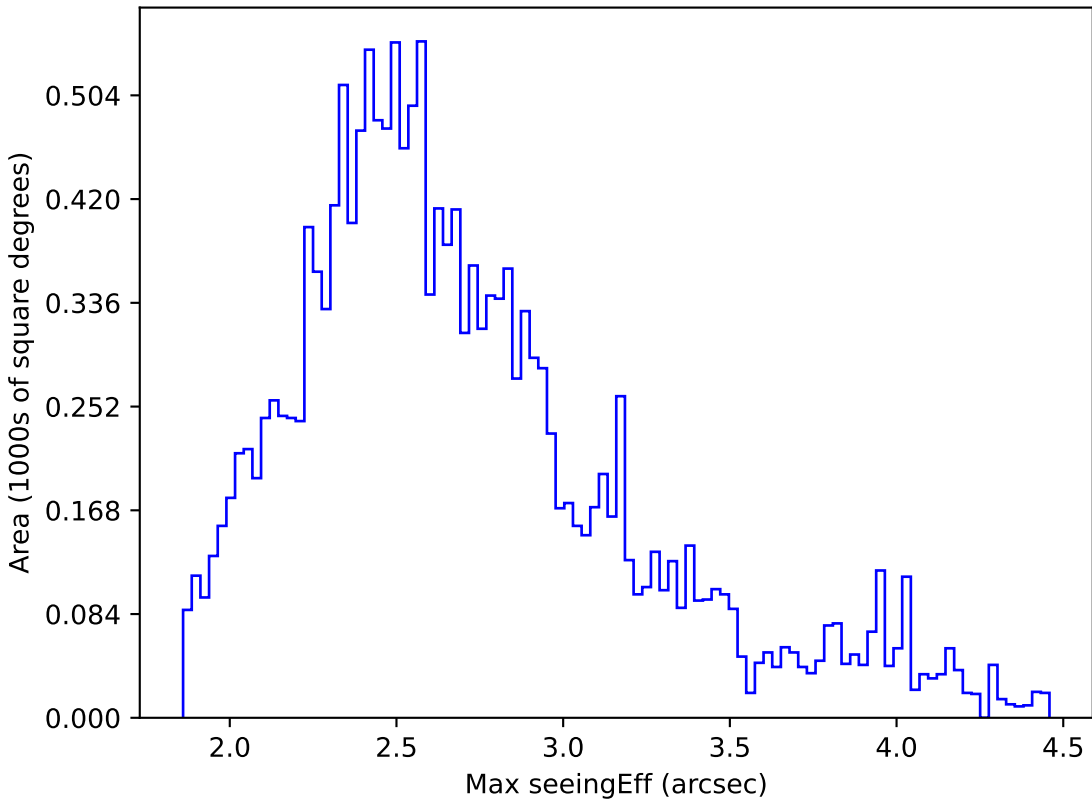
too_elab_r8_d2_gz_v3.4_10yrs WFD r band: Max seeingEff
