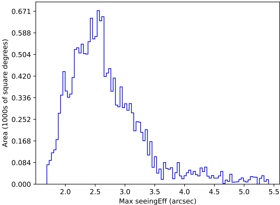
too_elab_r8_d2_gz_v3.4_10yrs WFD i band: Max seeingEff
