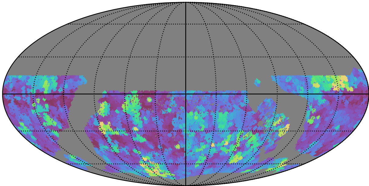
too_elab_r8_d2_gz_v3.4_10yrs WFD g band: Max seeingEff
