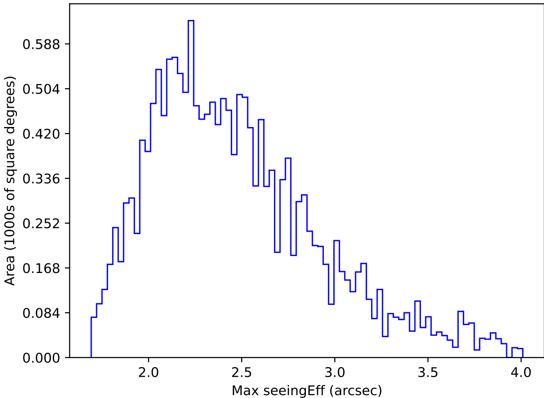
too_elab_r8_d2_gz_v3.4_10yrs WFD g band: Max seeingEff
