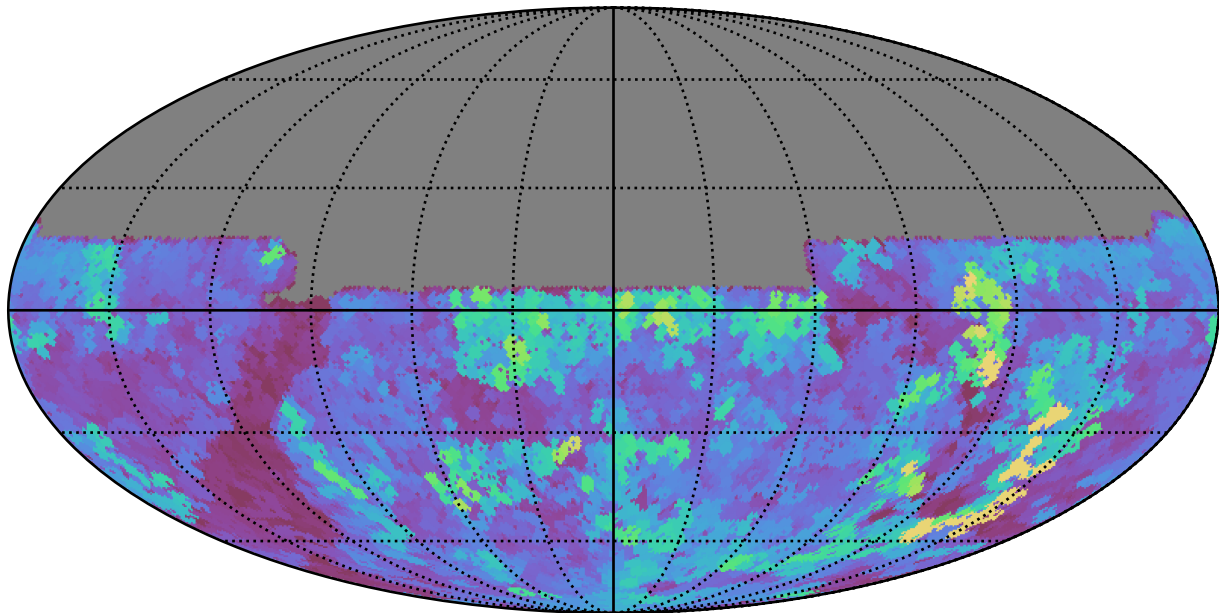
too_elab_r8_d2_gz_v3.4_10yrs All sky u band: Max seeingEff
