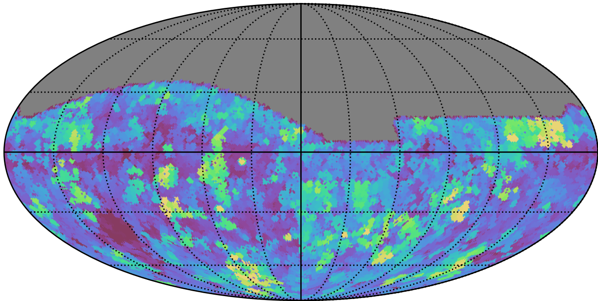
too_elab_r8_d2_gz_v3.4_10yrs All sky g band: Max seeingEff
