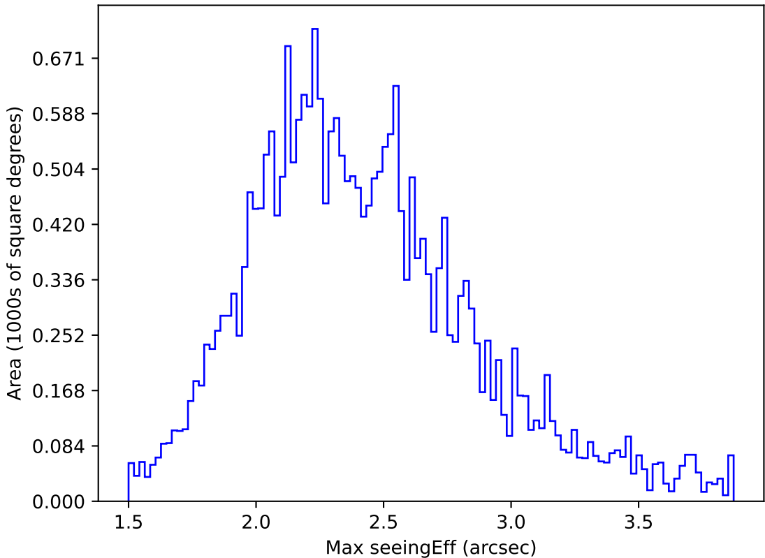
too_elab_r8_d2_gz_v3.4_10yrs All sky g band: Max seeingEff
