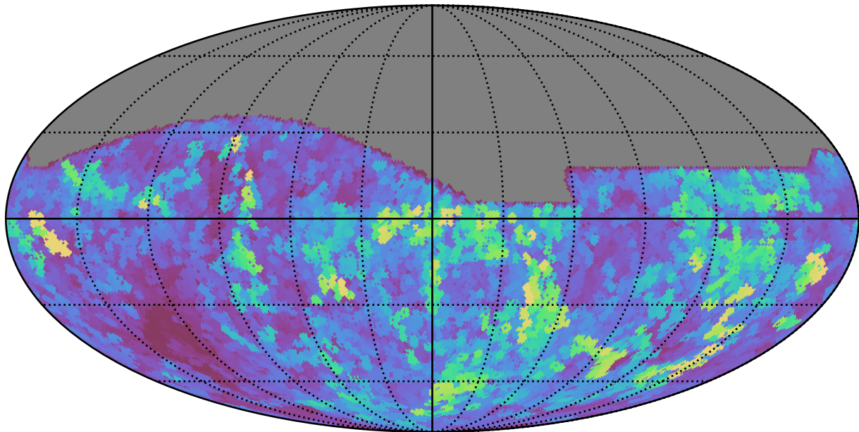
too_elab_r8_d2_gz_v3.4_10yrs All sky all bands: Max seeingEff
