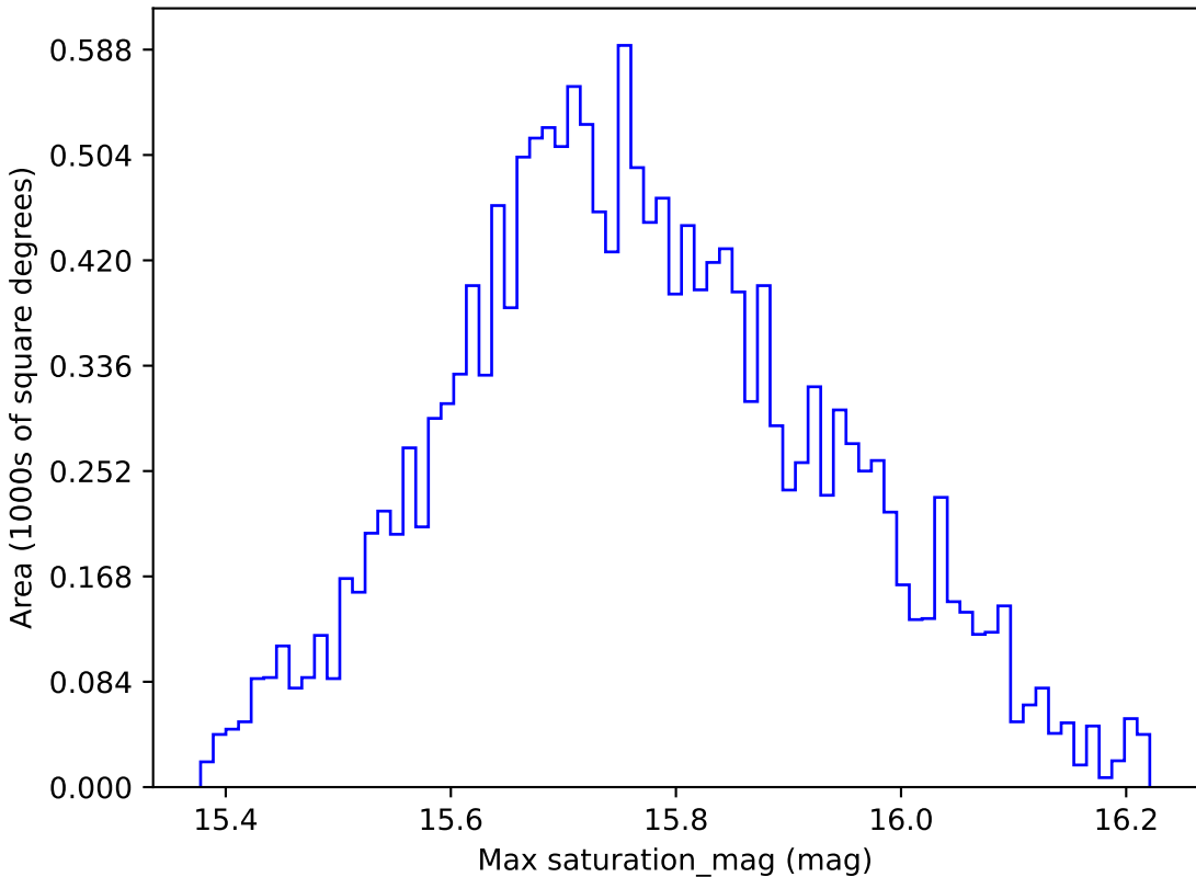
too_elab_r8_d2_gz_v3.4_10yrs WFD r band: Max saturation_mag
