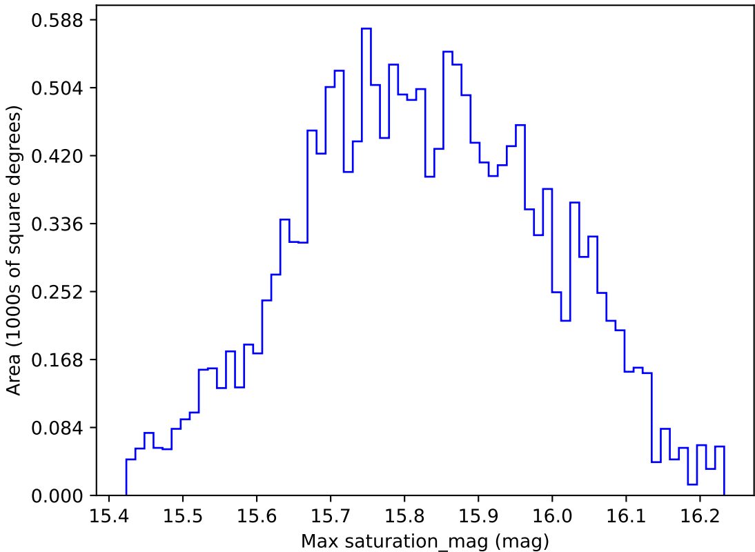
too_elab_r8_d2_gz_v3.4_10yrs WFD all bands: Max saturation_mag
